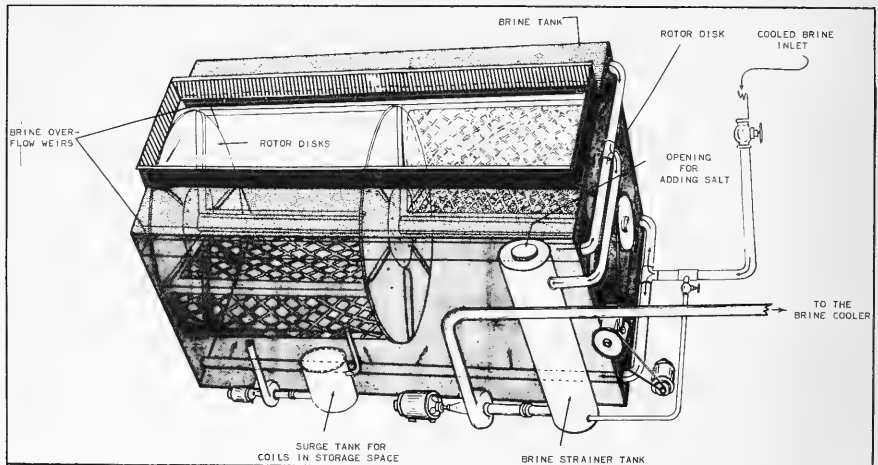
FIGURE 2 - BRINE-FREEZER TANK SHOWING ROTOR AND BRINE CIRCULATING EQUIPMENT.
